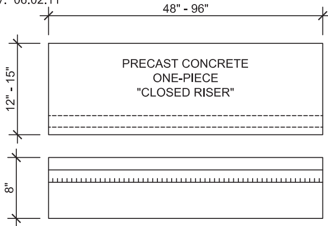
CLOSED RISER
